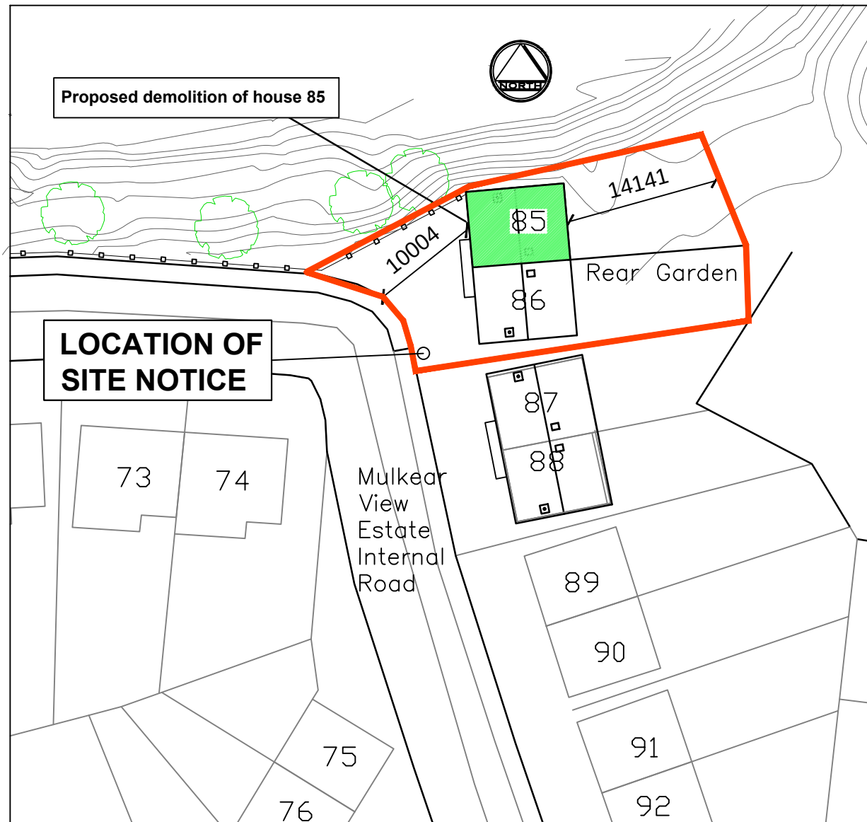
Existing Site Layout
